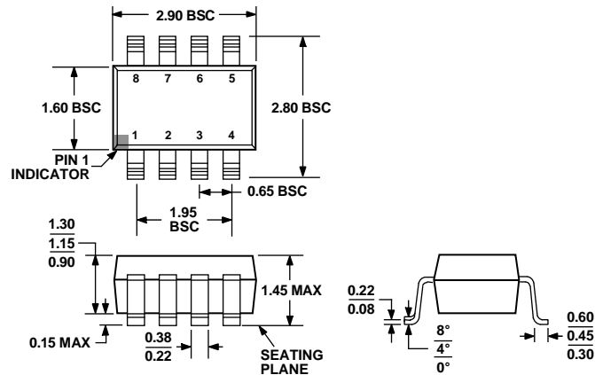
Figure 51. 8-Lead Small Outline Transistor Package [SOT-23] (RJ-8)
